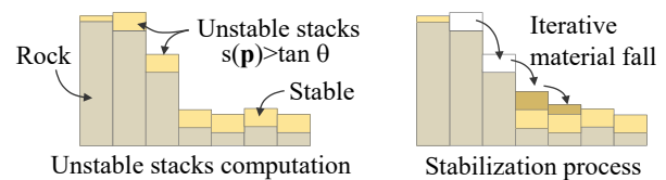
Figure 18: Overview of erosion: erosion occurs on piles whose slope is greater than the talus angle.
