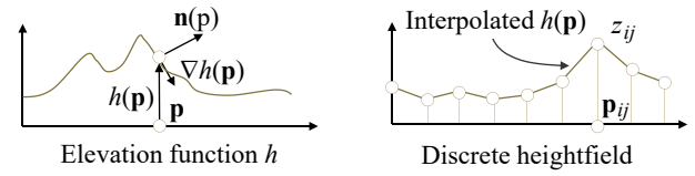
Figure 1: Elevation can be represented by an analytic or procedurally defined function, or by discrete heightfield data, in which case the elevation at any point is reconstructed by interpolation.
