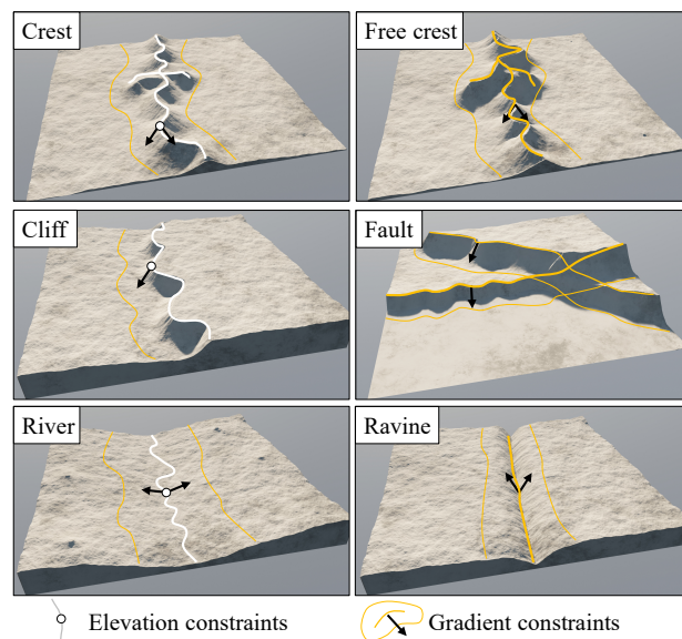
Figure 4: Using combinations of elevation and gradient constraints, a variety of geomorphological features can be authored.
