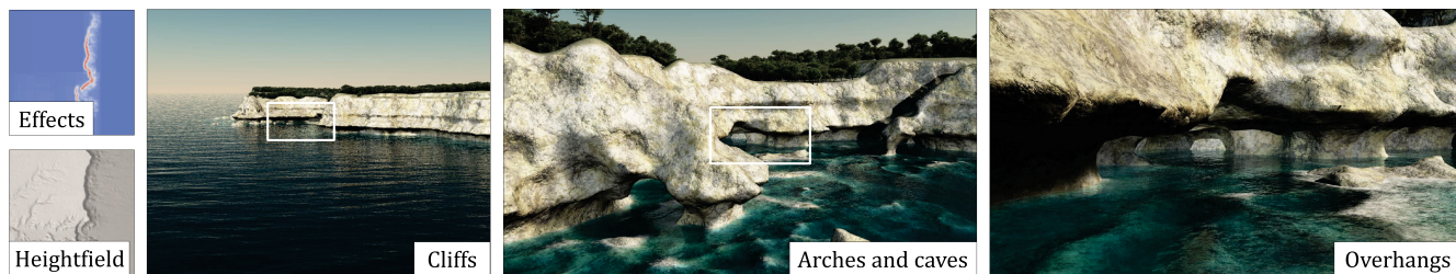
Fig. 11. An example of sea cliffs produced by our system. Starting from an input synthetic 2\frac{1}{2} D heightfield and geology with horizontal strata, we incrementally applied three steps of sea erosion. Sea action was limited to an 8-meter range either side of average sea level, leading to strong overhangs at the base of the cliff. Less durable rock area was specified in the geology model, which automatically generated the arch and sea cave. The effects inset shows the repartition of volumetric features on the terrain from a top view perspective.
