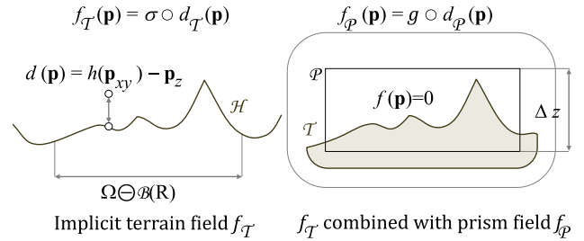
Fig. 6. Heightfield implicitization: given a C^1 elevation function h over a 2D domain \Omega \subset \mathbb{R}^2 , we construct a 3D primitive with field function f such that the implicit surface S = \{\mathbf{p} \mid f(\mathbf{p}) = T\} matches \mathcal{H} .
