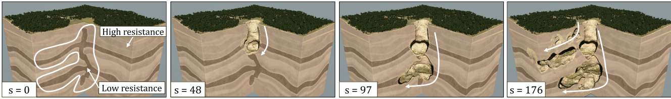
Fig. 13. Four steps in the generation of a cave system using a modified Invasion-Percolation algorithm. Starting from three sinks in the 2\frac{1}{2} D heightfield, invasion percolation progressively carves the subsurface of the terrain by following the least resistant layers of bedrock. Poisson Sphere sampling allows the creation of multiple tunnels.
