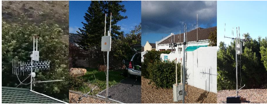
Figure 2: Outdoor measurements setup: (a) Static installation on roof (b, c) Mobile installation 500m up the road (d) Mobile installation 2.2 km away behind a tree
