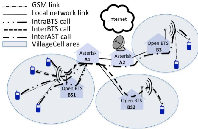
Figure 1: VillageCell network architecture. OpenBTS provides local coverage, while Asterisk nodes support call management and routing. The expected number of users, their spatial layout, and the local network traffic load are taken into account for OpenBTS and Asterisk interconnection and placement.
