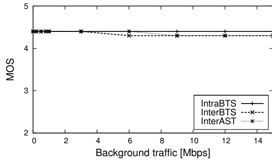
Figure 10: Mean opinion score (MOS) with varying level of background traffic.
