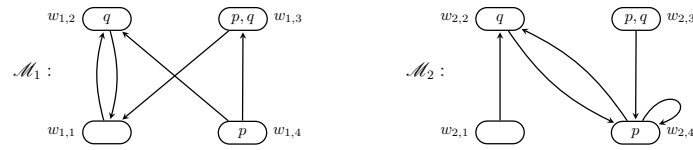
Fig. 1. Examples of Kripke models
